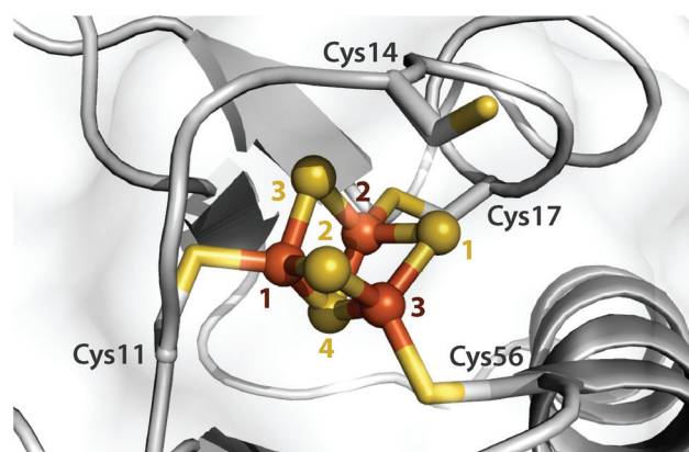
Fig. 1 [3Fe–4S] cluster of the ferricyanide-treated D14C ferredoxin from Pyrococcus furiosus . The cofactor inorganic core is shown in ball-and-stick representation. Sulfur and iron atoms are in yellow and brown, respectively. The cysteine at position 14 is facing away from the cluster. The presented crystal structure is based on chain A from PDB entry 3PNI. 8
