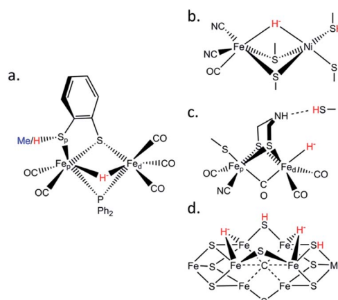
Fig. 1 Schematic structures of (a) the \mu\text{HS}(\text{Me}/\text{H}) synthetic complexes studied in this work; (b) the [NiFe] hydrogenase Ni–R intermediate; (c) the [FeFe] hydrogenase H hyd intermediate; (d) the nitrogenase Janus intermediate. The iron hydrides and sulfur protonations are labelled in red.
