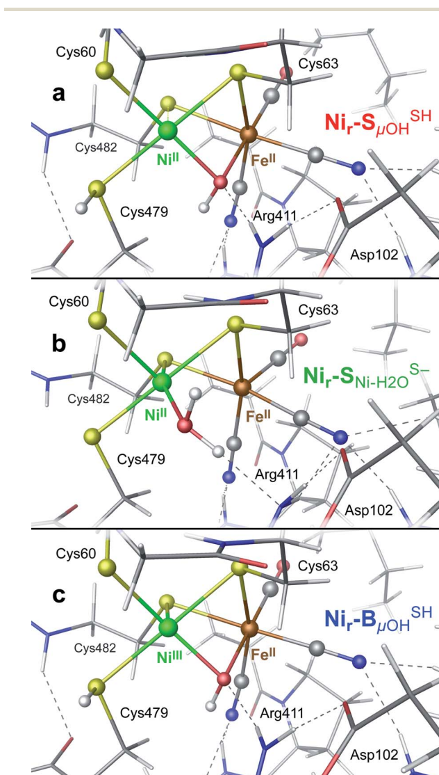
Fig. 3 DFT models: (a) \text{Ni}_r\text{-S}_{\mu\text{OH}}^{\text{SH}} of the reduced \text{Ni}_r\text{-S}_\text{I} state, (b) \text{Ni}_r\text{-S}_{\text{Ni-H}_2\text{O}}^{\text{S}^-} of the reduced \text{Ni}_r\text{-S}_\text{II} state, and (c) \text{Ni}_r\text{-B}_{\mu\text{OH}}^{\text{SH}} of the oxidized \text{Ni}_r\text{-B}'' state, displaying the [\text{NiFe}] cofactor metal ligands and their contacts with the nearby side chains in HoxC. For alternative models and the entire HoxC homology model employed, see Fig. S4–S10.†
