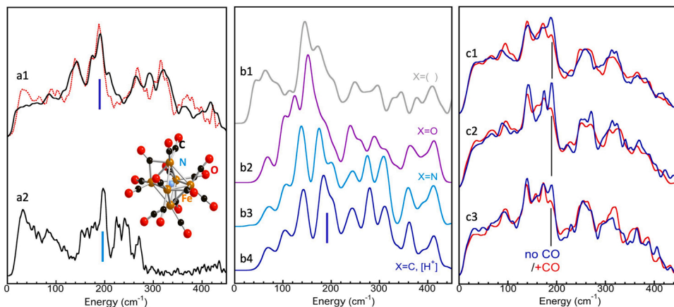
Fig. 9. (a1) NRVS of isolated FeMo-co (black) vs. M-center obtained via (MoFe protein – P cluster) difference spectrum (dashed red); (a2) NRVS of the model complex ion [Fe 6 N](CO) 15 3- while the right insert is the structure of this complex ion; (b) DFT calculated NRVS spectra assuming a central atoms of (b1) no atom, (b2) O, (b3) N, and (b4) C; (c) observed NRVS for a series of nitrogenase samples [(c1) wild type (WT); (c2) α-H195Q; (c3) photolysis product on WT, with CO (red) vs. without CO (blue) (For interpretation of the references to colour in this figure legend, the reader is referred to the web version of this article).
