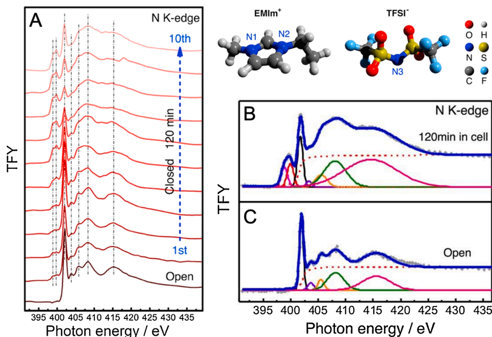
Fig. 7. (A) Time-lapsed experimental N K-edge XAS spectra acquired from an encapsulated ionic liquid sample with that acquired with the open ionic liquid droplet in vacuum (bottom). Peak deconvolution of N K-edge spectra collected in (B) in the closed geometry after 120 min exposure and (C) in the open geometry. Adapted from Ref. [53] with permission from the American Chemical Society.
