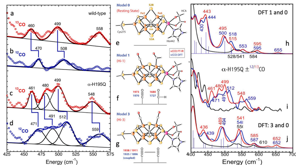
Fig. 10. NRVS of ^{13}\text{CO} (a) and CO (b) bound wild type (WT) nitrogenase vs. ^{13}\text{CO} (c) and CO (d) bound \alpha -H195Q nitrogenase in the Fe—CO region (425–575 \text{cm}^{-1} ); Structural models 0 (e), 1 (f) and 3 (g) used for DFT calculation on NRVS of as-isolated, WT + CO and \alpha -H195Q + CO nitrogenases respectively; DFT calculated (or observed) NRVS for as-isolated (black) vs. CO (blue) and ^{13}\text{CO} (red) bound nitrogenases: (h) DFT calculation on WT and WT + CO using model 0 (black) and 1 (blue and red); (i) observed NRVS for \alpha -H195Q nitrogenase (black), + CO (blue) and + ^{13}\text{CO} (red); and (j) DFT calculation on \alpha -H195Q and \alpha -H195Q + CO using model 0 (black) and 3 (blue and red) (For interpretation of the references to colour in this figure legend, the reader is referred to the web version of this article).
